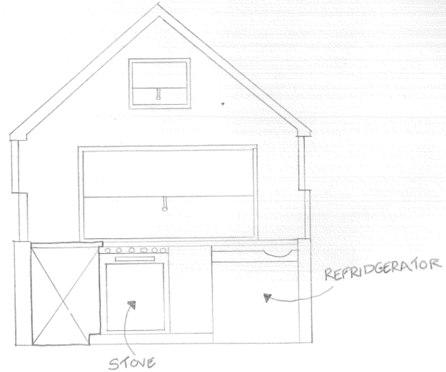
② SOUTH ELEVATION
