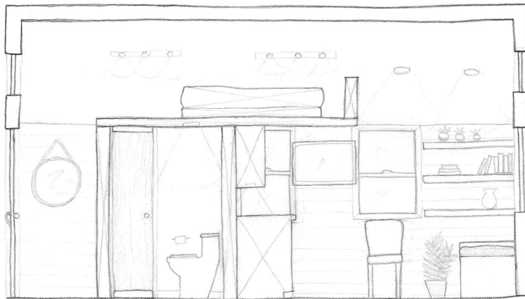
E4 LEFT WALL ELEVATION SCALE \frac{1}{2}'' = 1'-0''
