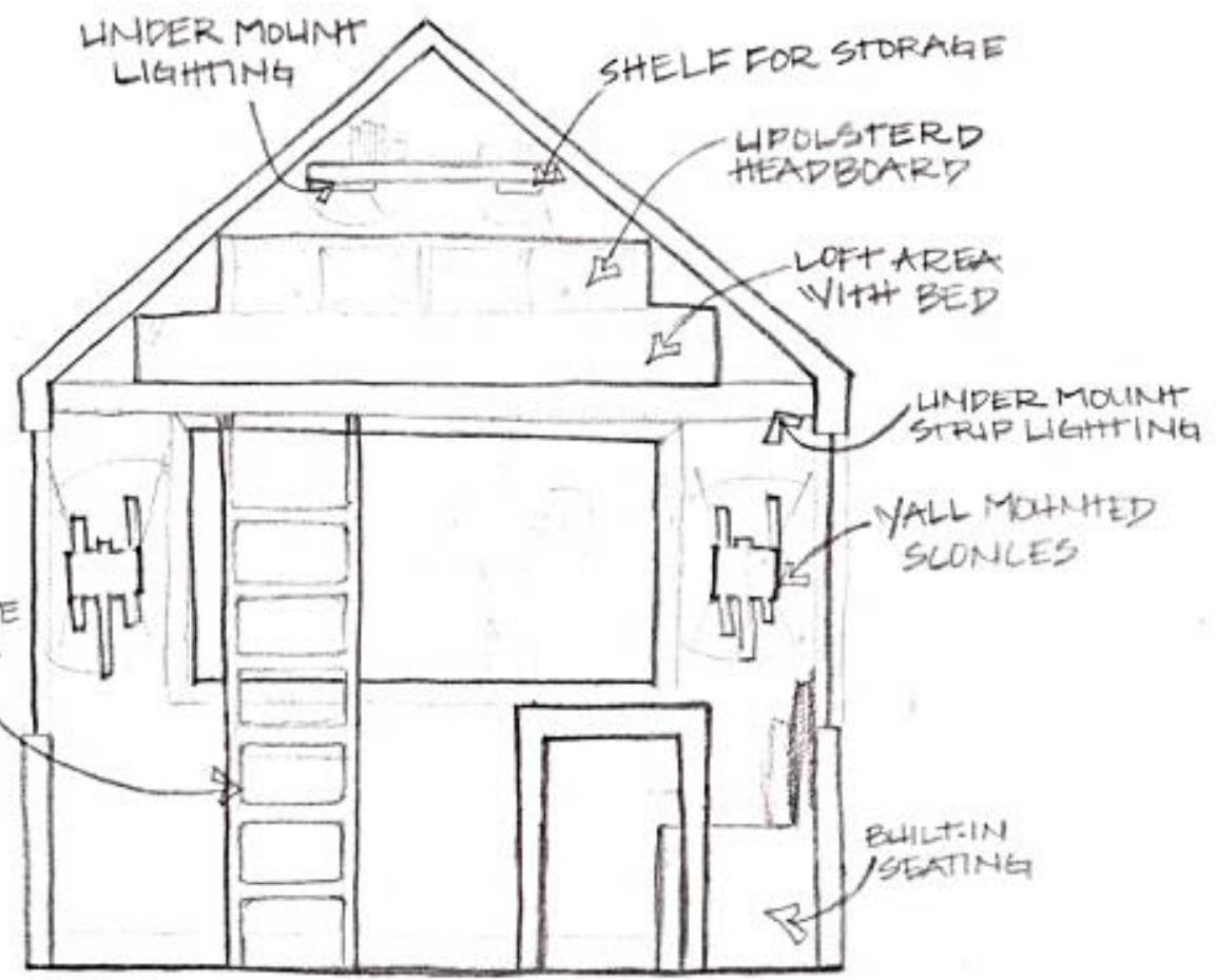
LOFT + EATING ELEVATION
