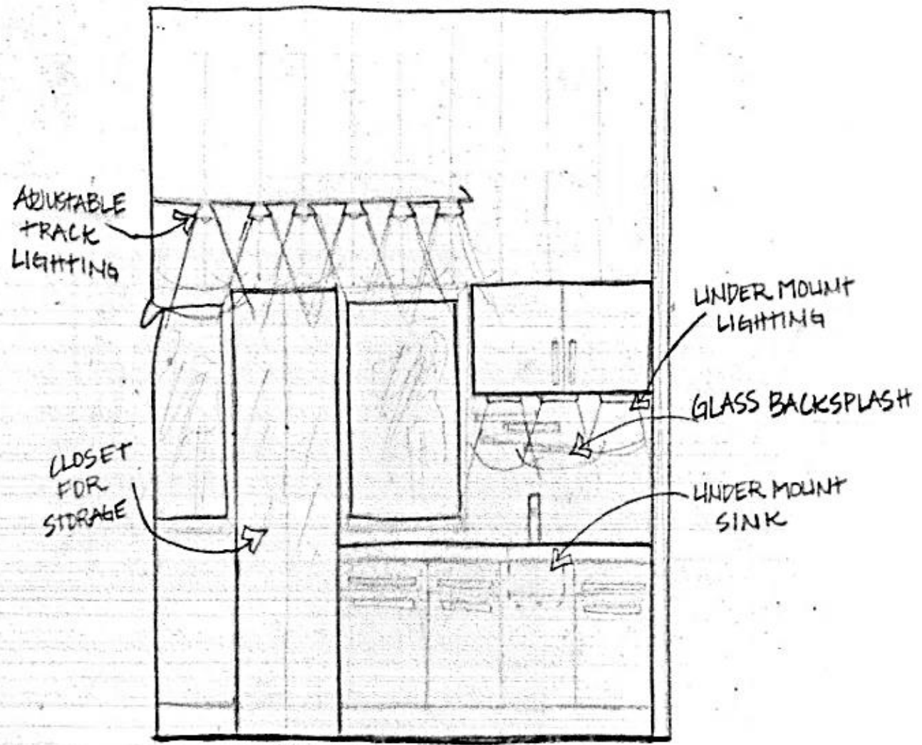
KITCHEN ELEVATION
